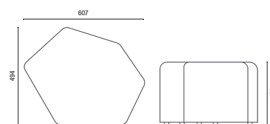
36445 Hexagonal Irregular Médio 450mm
