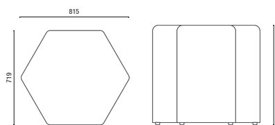
36675 Hexagonal Regular Alto 750mm
